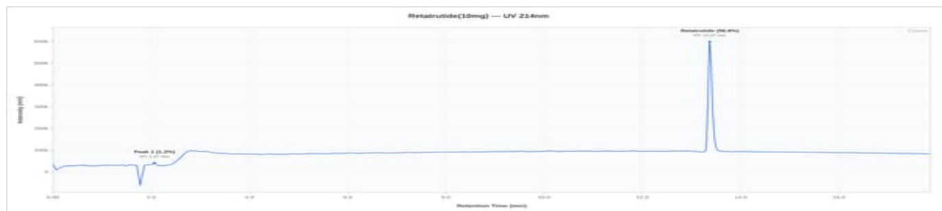
RETA-3 10mg - PL1004: UV Chromatogram
