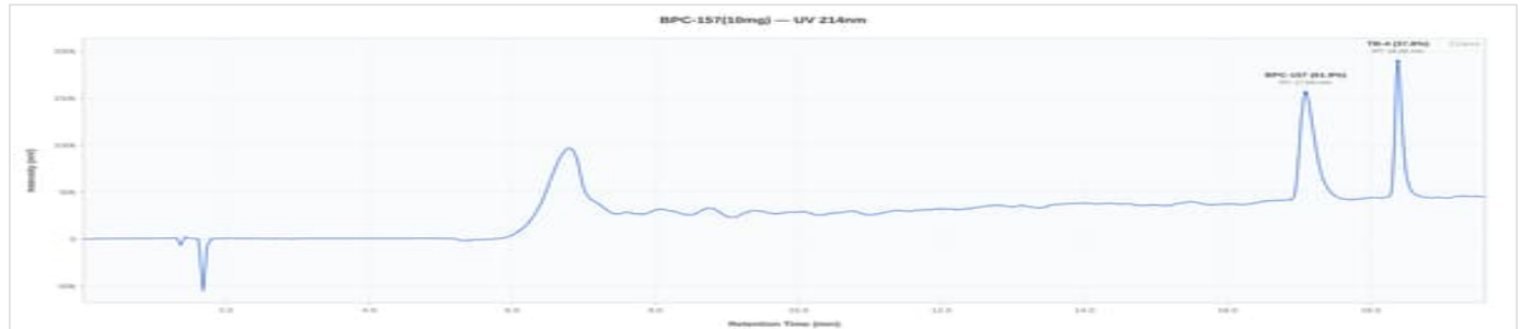
BPC-157 / TB-500 10mg - PL1007: UV Chromatogram
