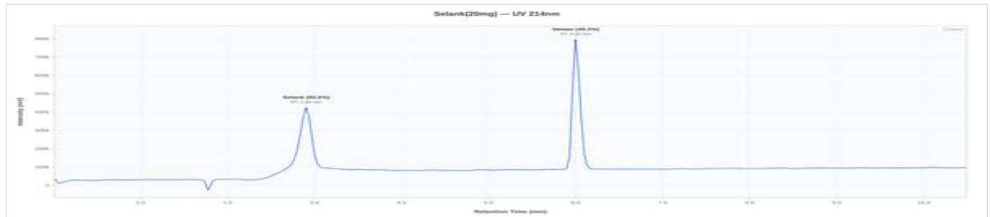
SEMAX/SELANK 20mg - PL1008: UV Chromatogram
